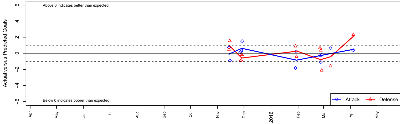
Utah FC 00 Premier G99 Dots are actual minus expected GF (blue circles) and GA (red triangles). Blue line is smoothed change in attack strength. Red is smoothed change in defense strength.
